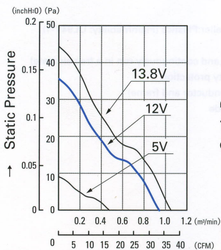
→ Air Flow 9S0812F402(4021)
