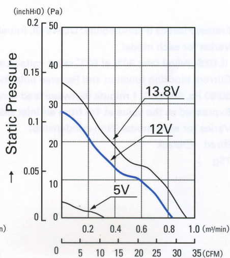
→ Air Flow 9S0812M402(4021)
