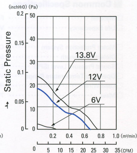
→ Air Flow 9S0812L402(4021)
